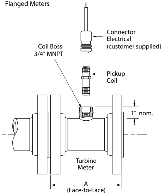
Flanged Meter Face-to-Face Dimensions (Dim. A)
